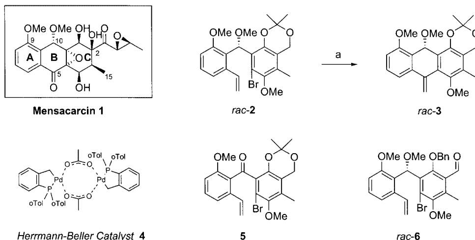
Scheme 1. Mensacarcin ( 1 ), synthesis of tetrahydroanthracene rac -3 and structures of substrates rac -2, 5 and rac -6: (a) n Bu 4 NOAc, DMF/CH 3 CN/H 2 O, 60 °C then HB cat 4 , 120 °C, 4 h, 24%.
