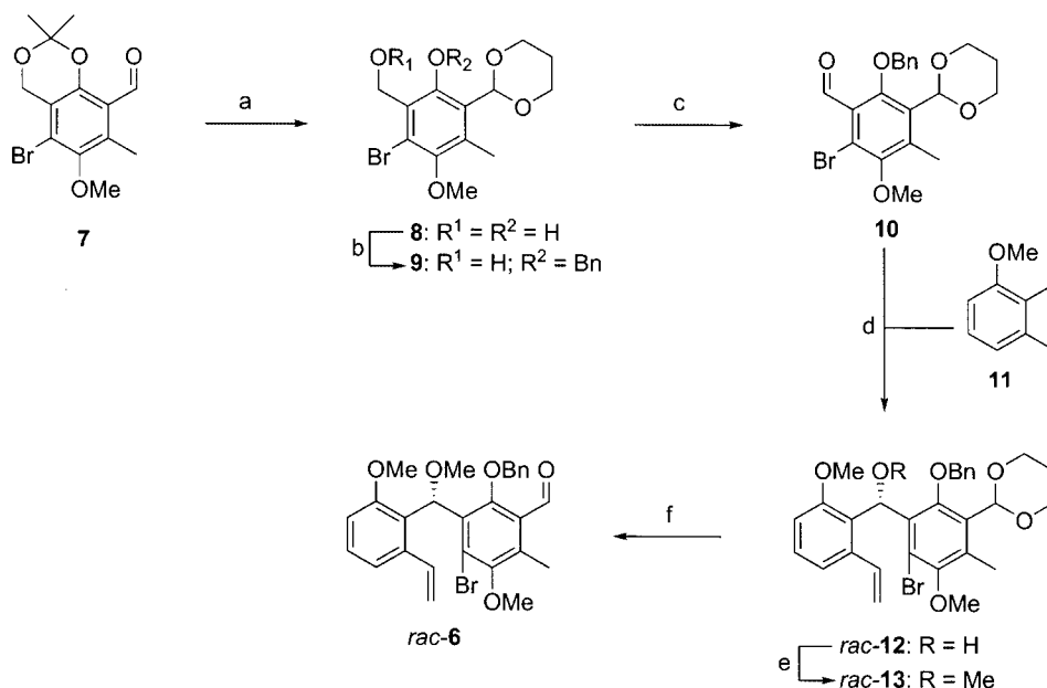
Scheme 2. Synthesis of diphenylcarbinol rac-6 : (a) i) AcOH, 60 °C, 4 h, 66%; ii) 1,3-propanediol, Amberlyst 15 H + , C 6 H 6 , reflux, 5 h, 98%; (b) BnBr, K 2 CO 3 , CHCl 3 /MeOH, 40 °C, 12 h, 80%; (c) Dess–Martin periodinane, CH 2 Cl 2 , 1 h, 81%; (d) iodobenzene 11 , n BuLi, THF, –78 °C, 20 min then 10 , THF, –78 °C, 20 min, 20 °C, 39%; (e) KH, THF, 0 °C, 40 min then MeI, 20 °C, 1 h, 91%; (f) PPTS, H 2 O/acetone, reflux, 12 h, 71%.
